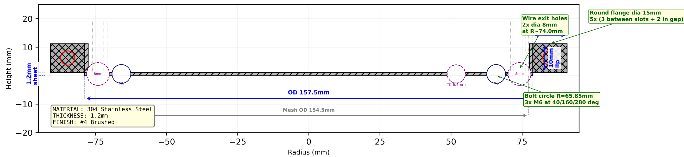
CROSS SECTION (through screw tab center)
